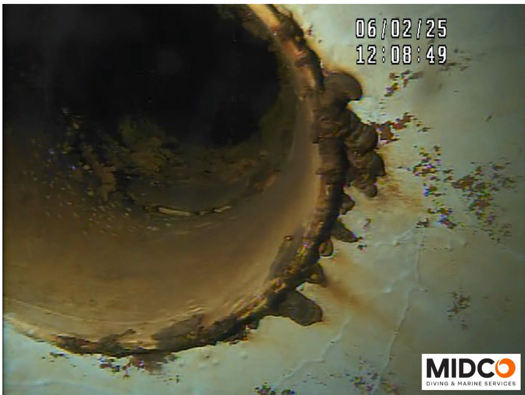
Inlet Plumbing – Coating Failure with Corrosion Noted
