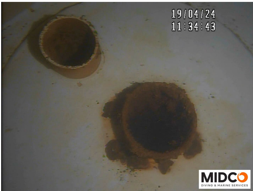
Interior Plumbing #1 & #2 – Coating Failure with Corrosion Noted
