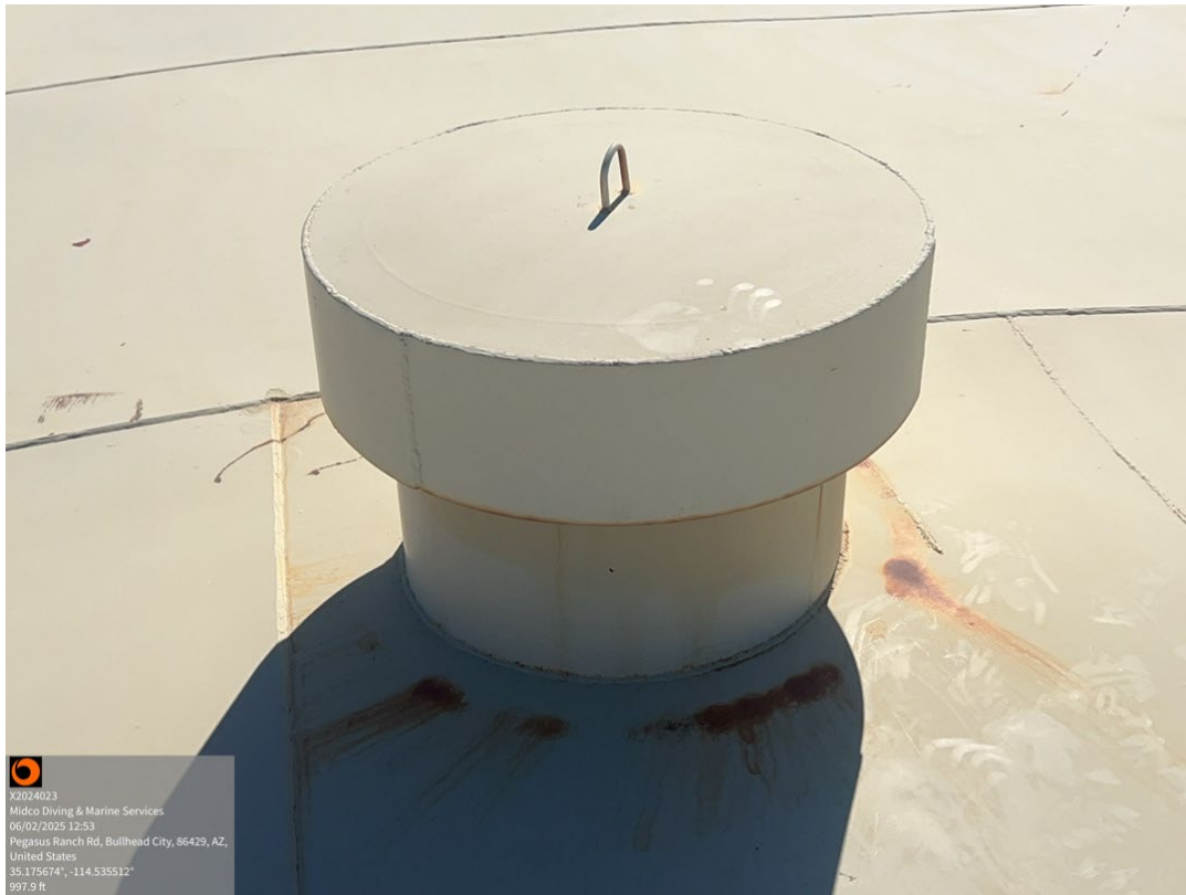
Roof Vent – Coating Failure with Corrosion Noted
