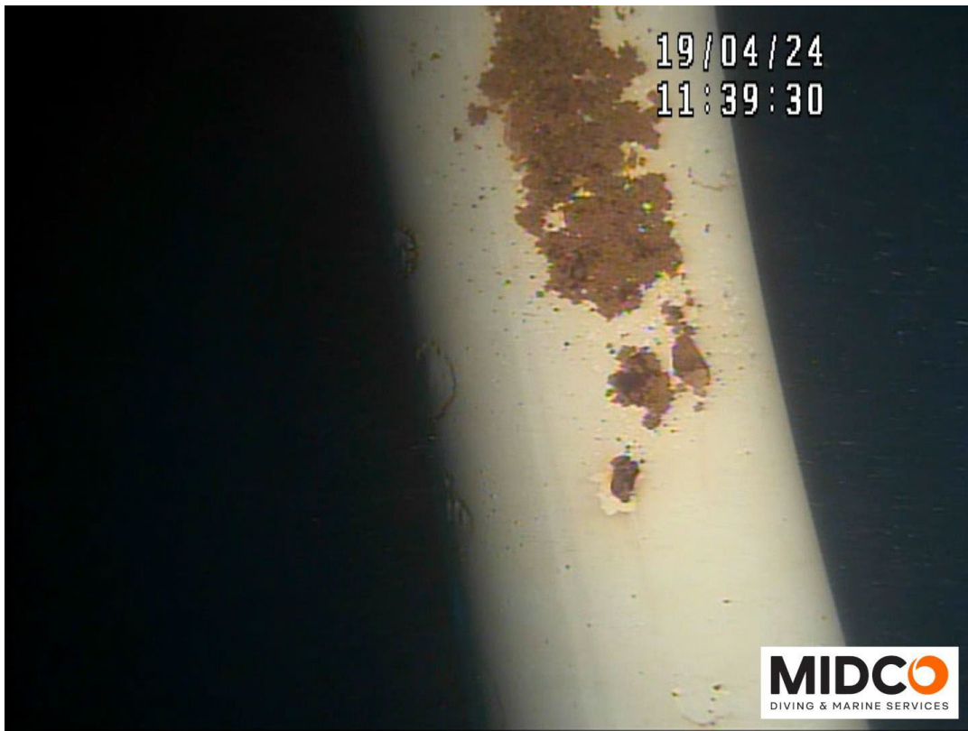
Support Column – Coating Failure with Corrosion Noted
