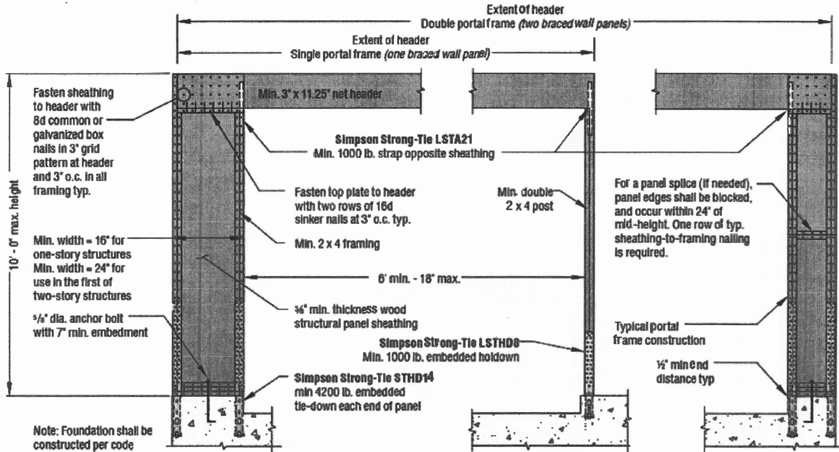
Method PFH: Portal Frame with Holdowns
